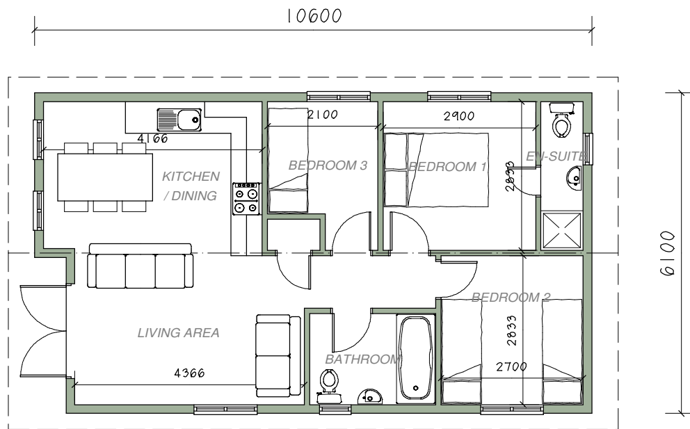
FLOOR PLAN
