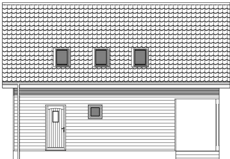
SIDE ELEVATION
