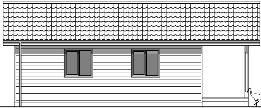
SIDE ELEVATION
