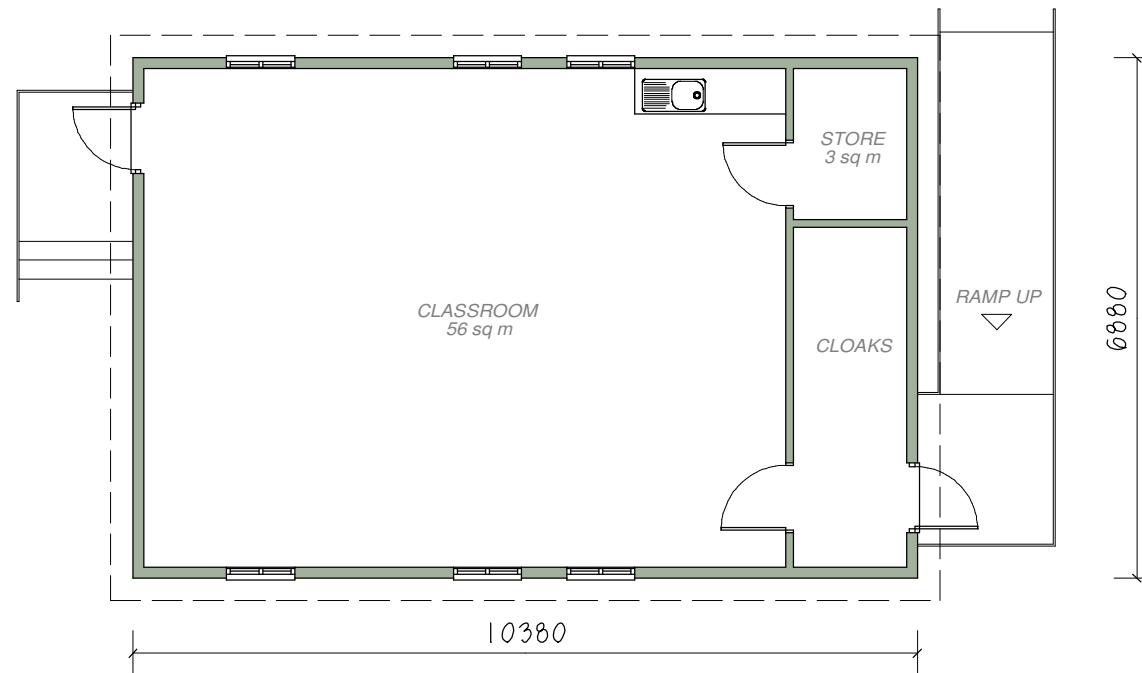
FLOOR PLAN
